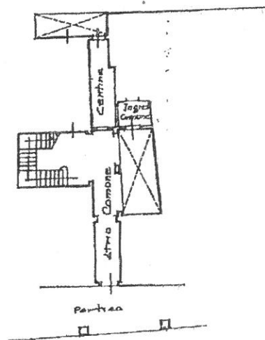
PIANO TERRA
